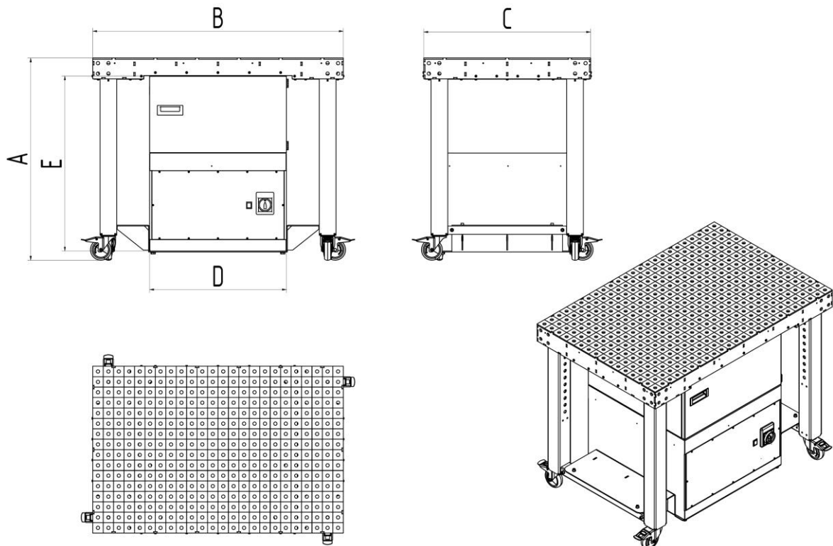
Fig. 19: Dimensions sheet
