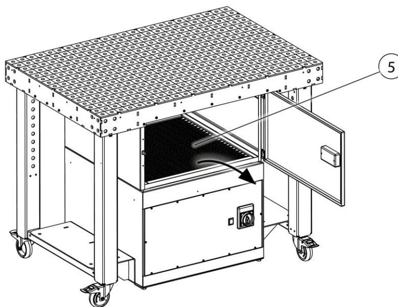
Fig. 16: Filter change – activated charcoal filter (optional)
