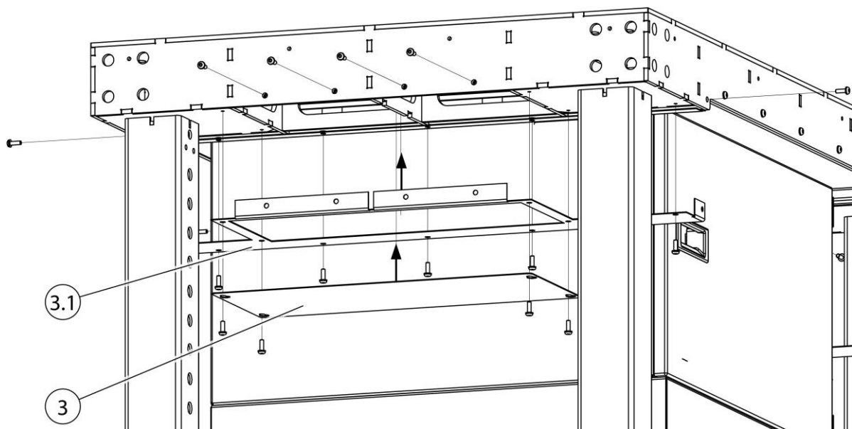
Fig. 10: Installation - Dust pan
