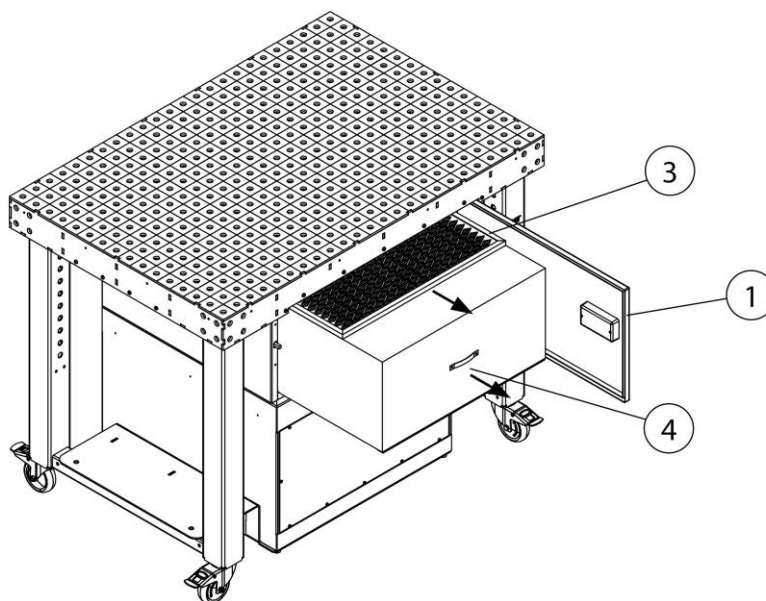
Fig. 12: Checking the direction of fan rotation
