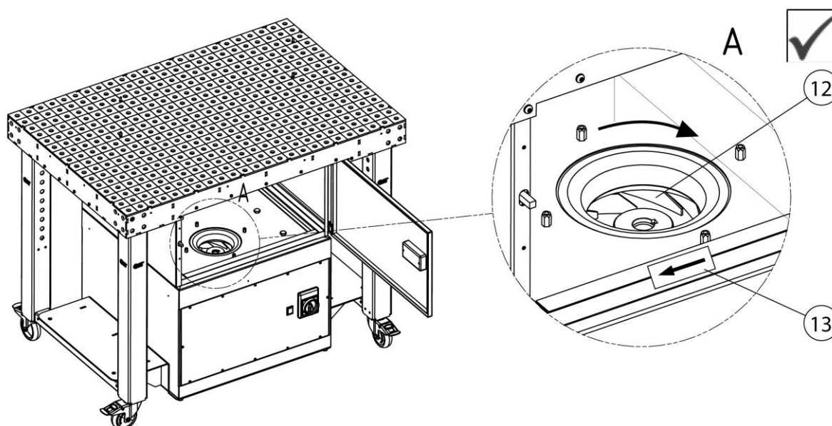
Fig. 13: Checking the direction of rotation of the fan impeller
