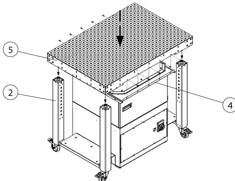
Fig. 8: Installation - Table top
