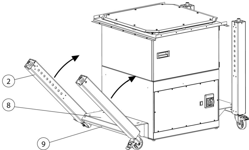
Fig. 7: Installation - Table legs
