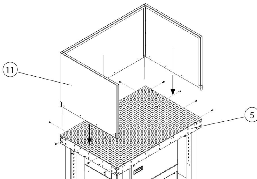
Fig. 11: Installation – side wall (optional)
