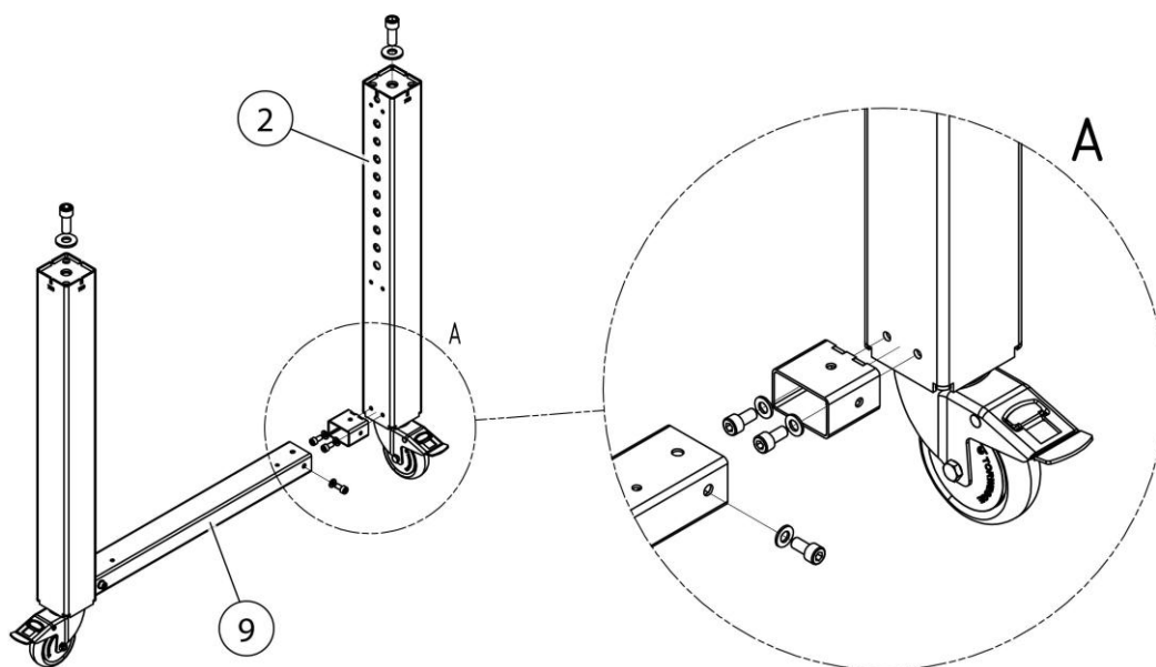
Fig. 6: Installation - Table legs
