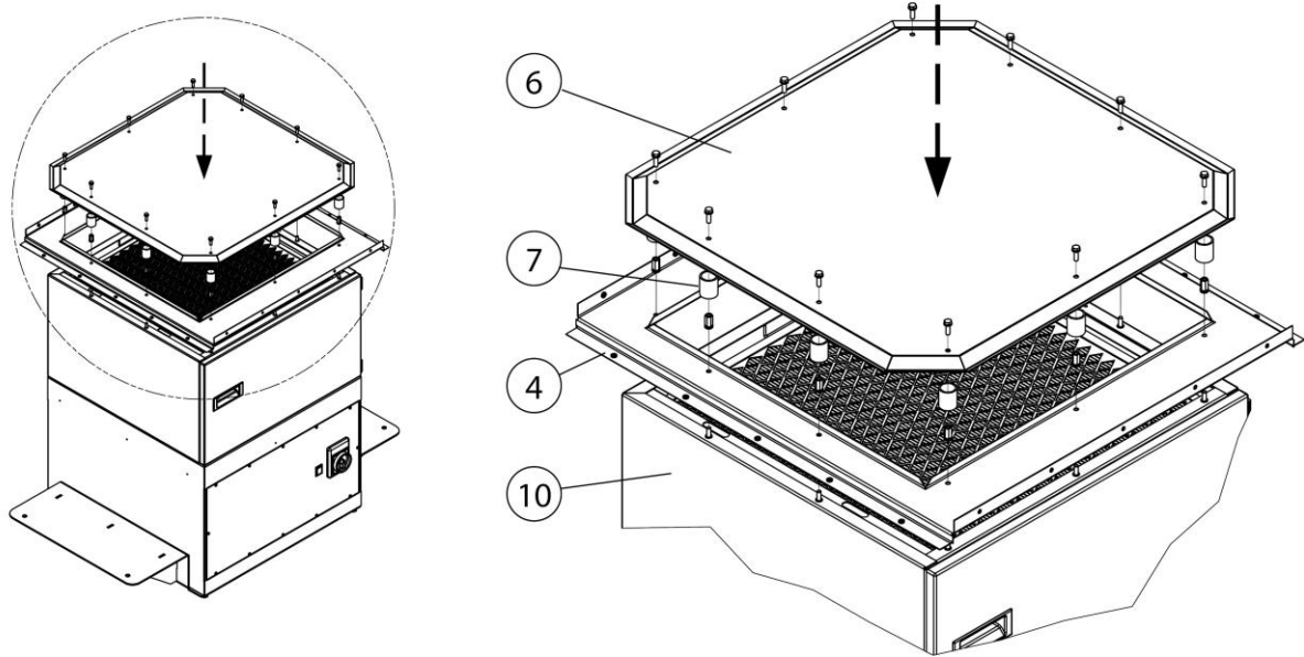
Fig. 5: Installation - Support frame + spark plate
