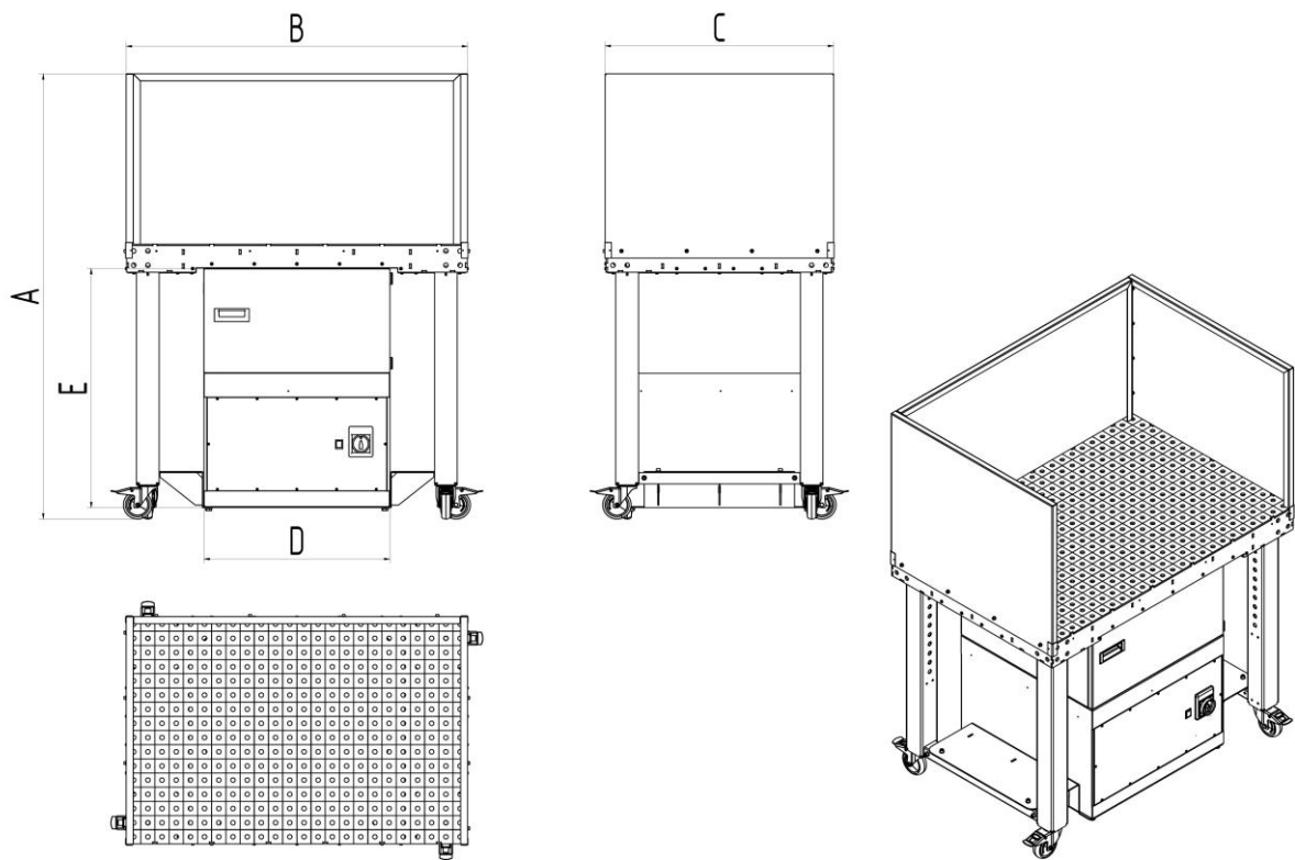
Fig. 20: Dimension sheet with side wall
