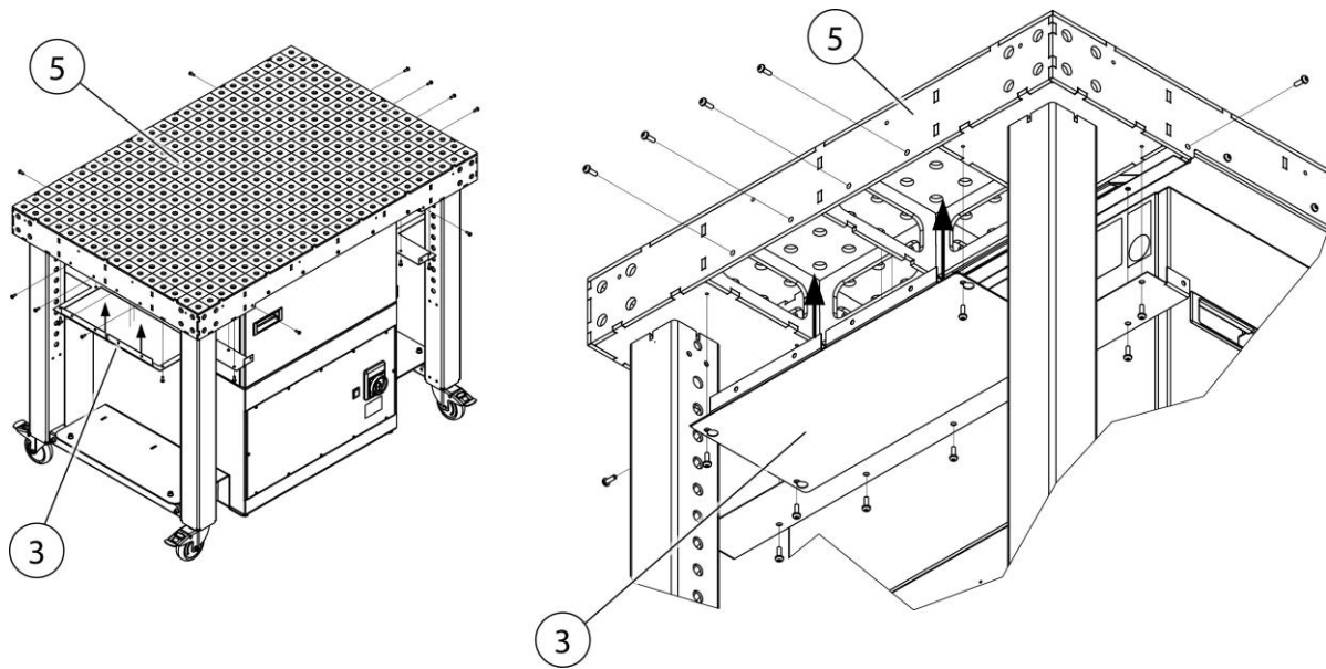
Fig. 9: Installation - Dust pan
