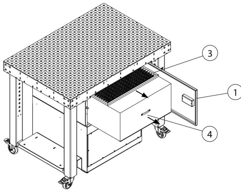
Fig. 15: Filter change – pre-filter + main filter
